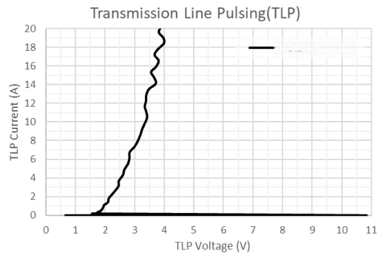
Figure 4. TLP(1/100ns)
